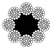
8 x 41 WS FC 1+8+8/8+16
