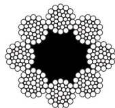
8 x 36 WS FC 1+7+7/7+14
