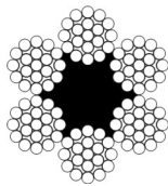
6x19S FC (1-9-9)
