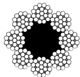
8 x 25 F FC 1+6+6F+12
