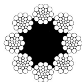
8 x 26 WS FC 1+5+5/5+10
