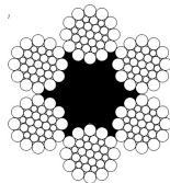
6 x 41 WS AT/FC 1+8+8/8+16
