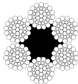
6 x 36 WS AT/FC 1+7+7/7+14
